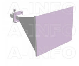
LB-90-20-C-TFSP Standard Gain Horn Antenna 8.2-12.4GHz 20dB Gain TNC Female
